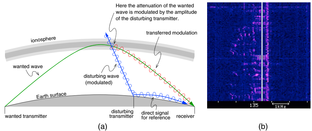
Figure 1. (a) Sketch of how ionospheric cross modulation happens. (b) Spectrogram (from Vester, 2013) on the Twente WebSDR showing the first case of sideband asymmetry; horizontal frequency, vertical time (about 15 s), brightness represents signal strength; the 135.43 kHz transmitter was unmodulated. (The WebSDR is a web-controlled receiver at http://websdr.ewi.utwente.nl:8901/ , capable of tuning from 0 to 29 MHz independently by hundreds of simultaneous users; in fact, the Twente receiver referred to later is this same system.)
