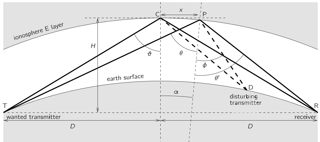
Figure 9. Geometry of the deflected-ray explanation.
