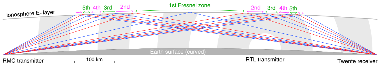
Figure 6. Sketch illustrating a qualitative explanation of the sideband asymmetry.
