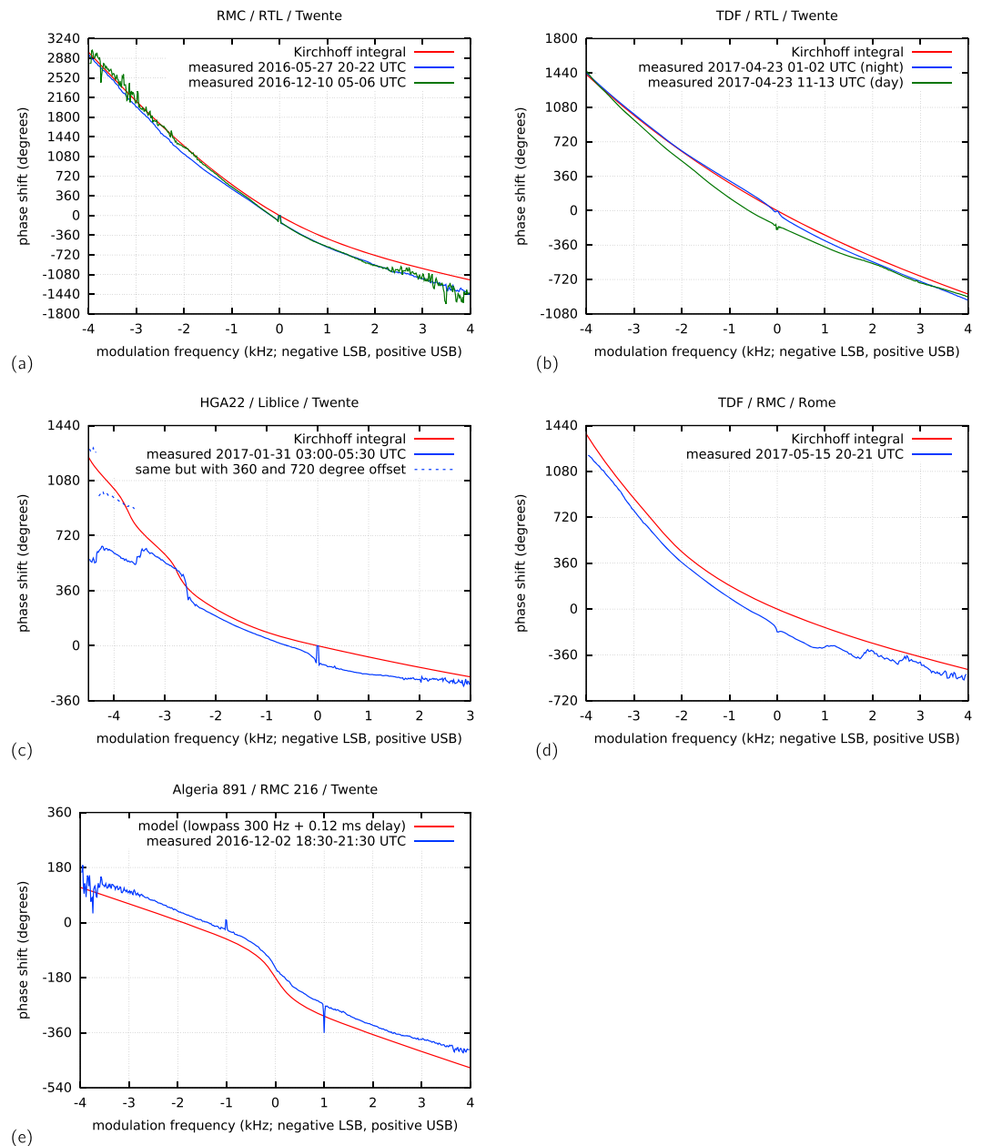
Figure 5. Comparison of phase as measured and as calculated using the Kirchhoff integral in (a)–(d); (e) shows a case without asymmetry for reference. LSB = lower sideband; USB = upper sideband.
