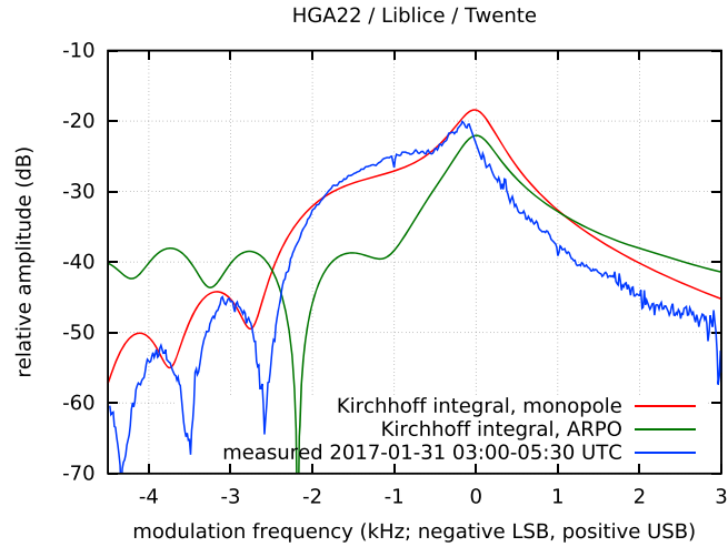
Figure 10. Measured and modeled amplitude behavior in the HGA22/Liblice/Twente case. LSB = lower sideband; USB = upper sideband.
