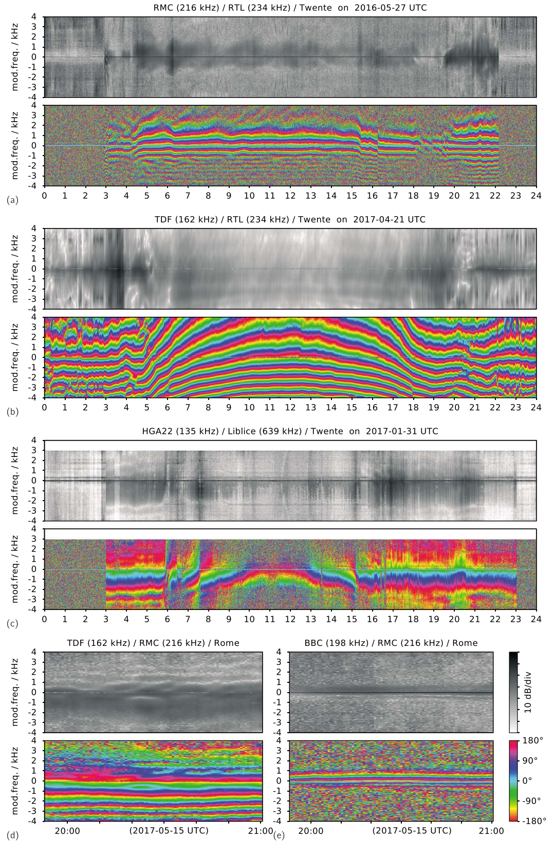
Figure 4. Typical exploratory measurement results, showing the magnitude (darker = larger) and phase (color scale at bottom right) of the ionospheric cross modulation separately for both sidebands. (a)–(e) are for several combinations of transmitters and receivers.
