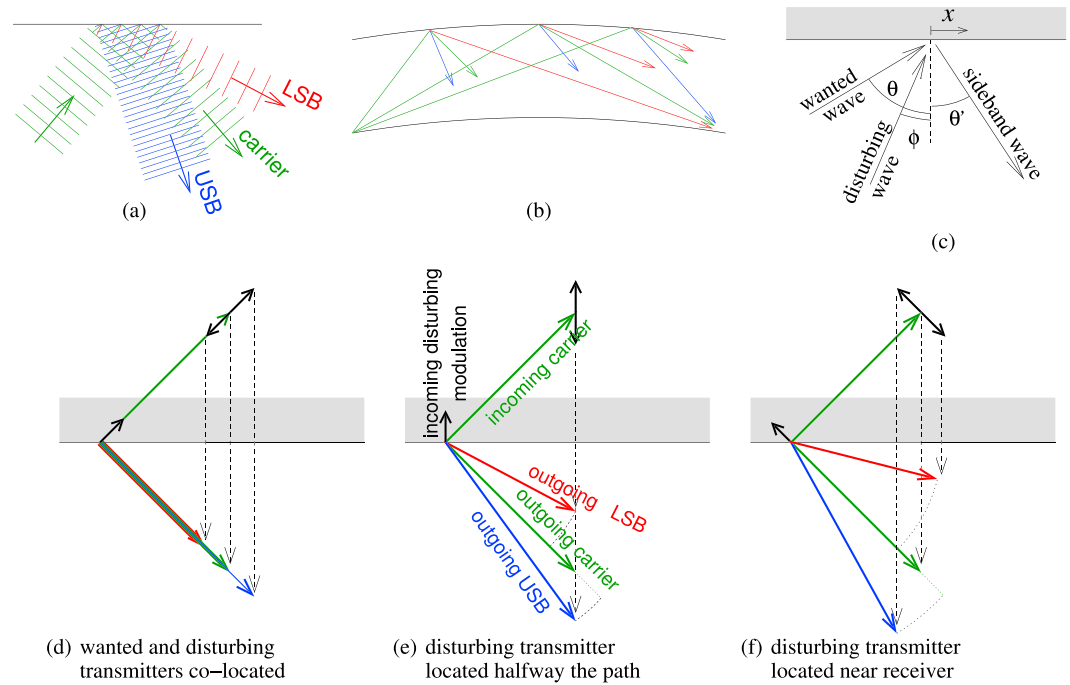
Figure 7. Essence of the deflected-ray explanation. (a) Reflection at one point of the ionosphere; (b) reflections as seen by one receiver; (c) calculation of reflection angle; (d)–(f) wave vectors in three cases.
