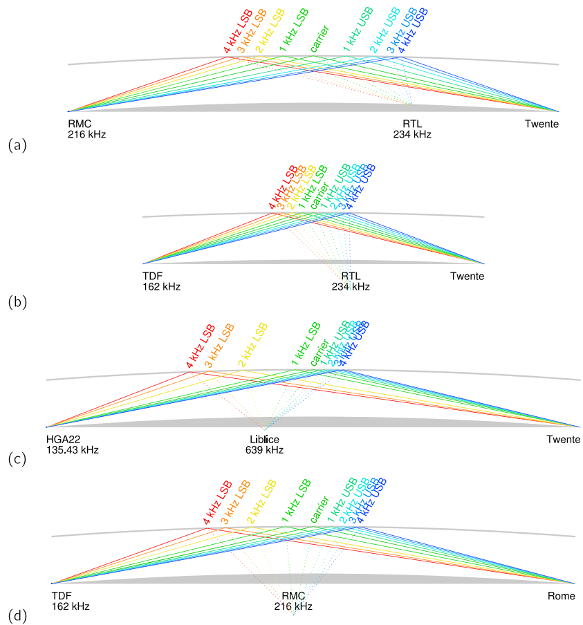
Figure 8. Ray tracing for the various examples. (a)–(d) correspond to the cases of Figures 4a–4d and 5a–5d.
