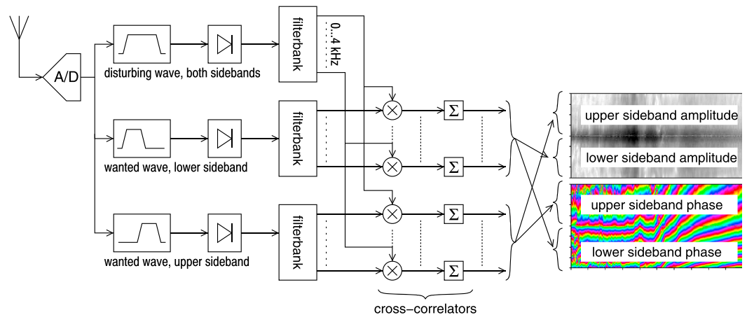
Figure 2. Measurement setup.
